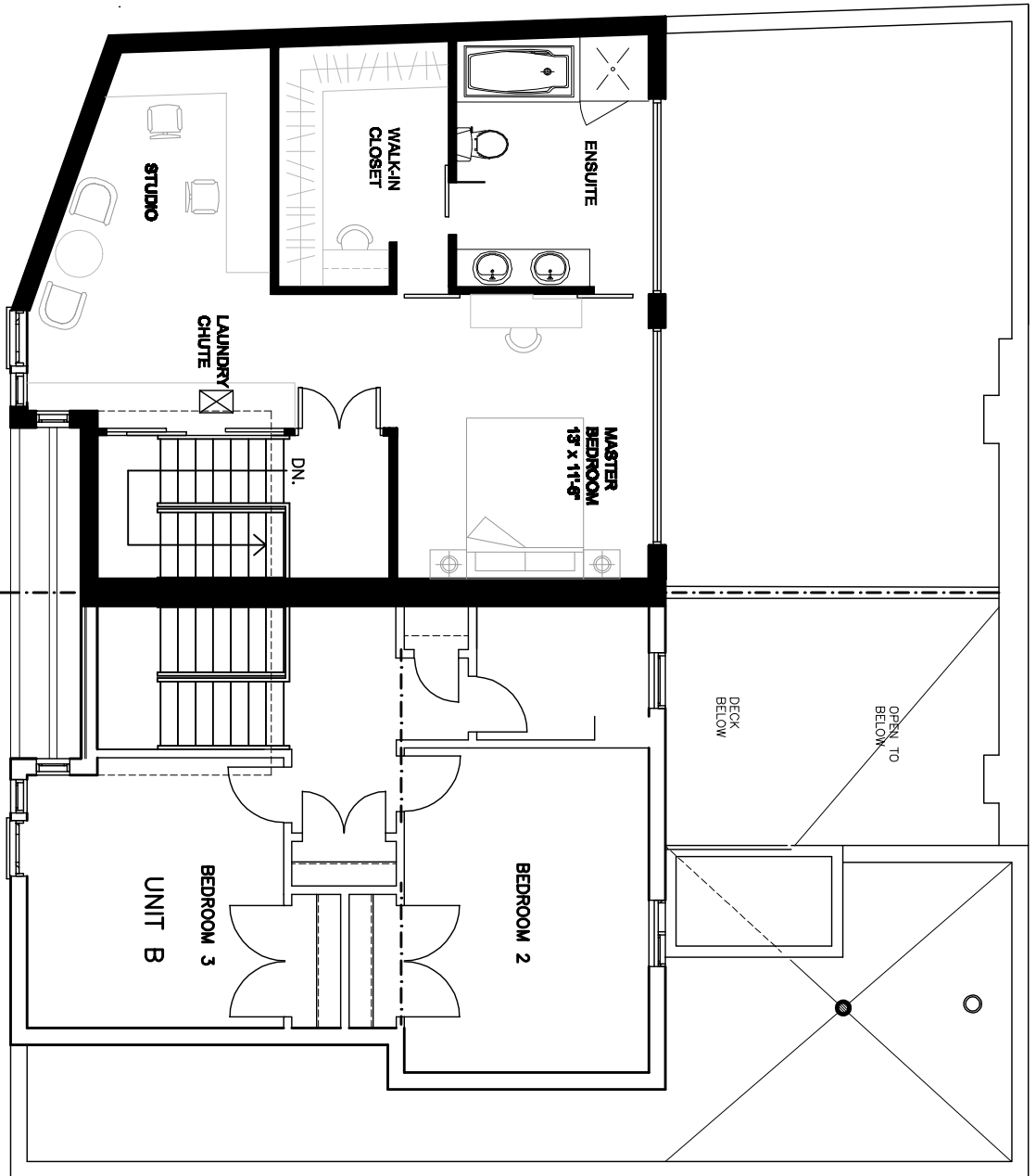
1 A1.2 Scheme A THIRD FLOOR PLAN 3/16" = 1'-0"
